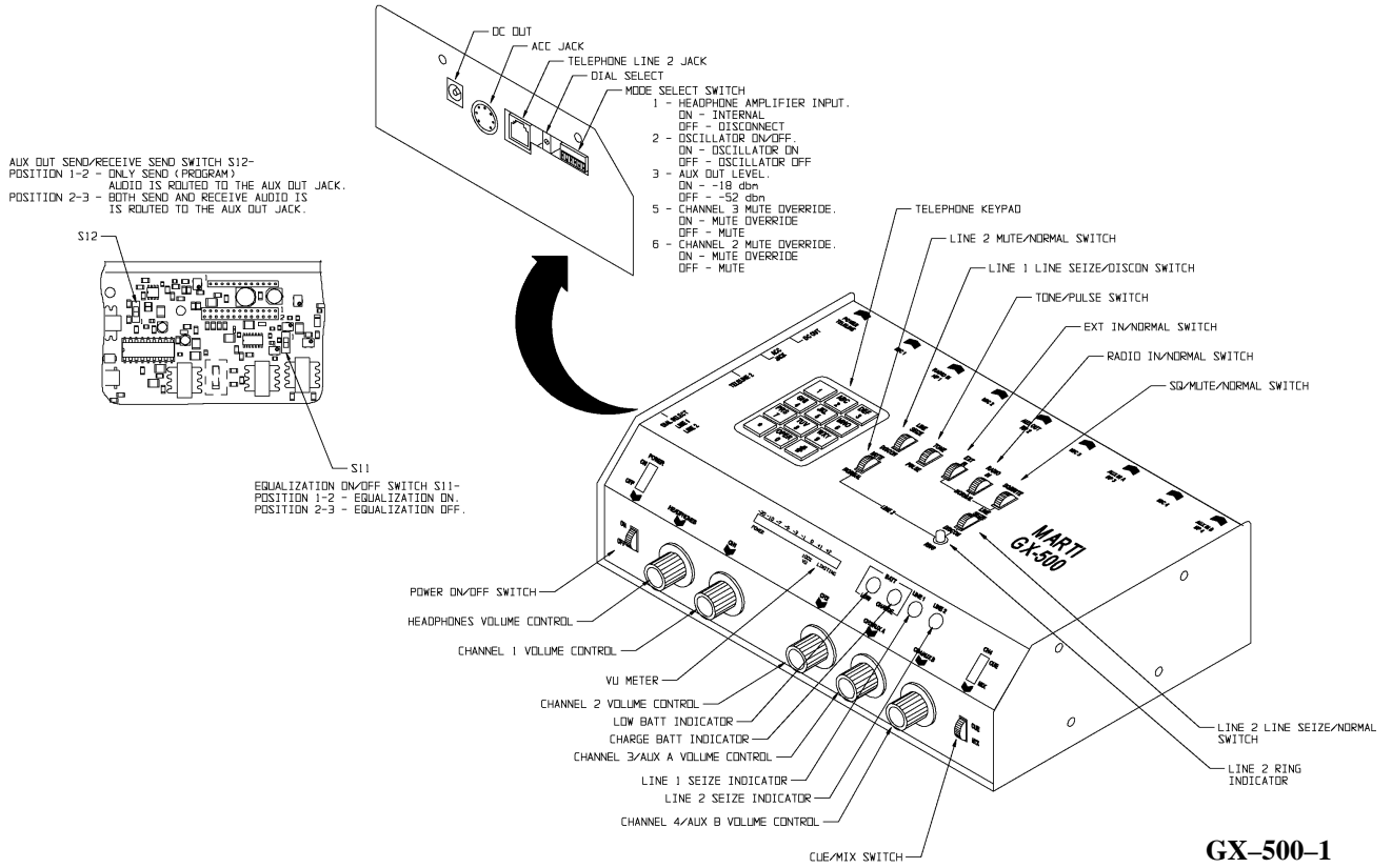
FIGURE 1. GX-500 CONTROLS AND INDICATORS (Sheet 1 of 3)
