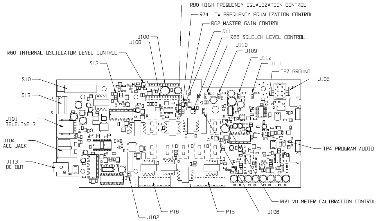
FIGURE 1. GX-500 CONTROLS AND INDICATORS (Sheet 3 of 3)
