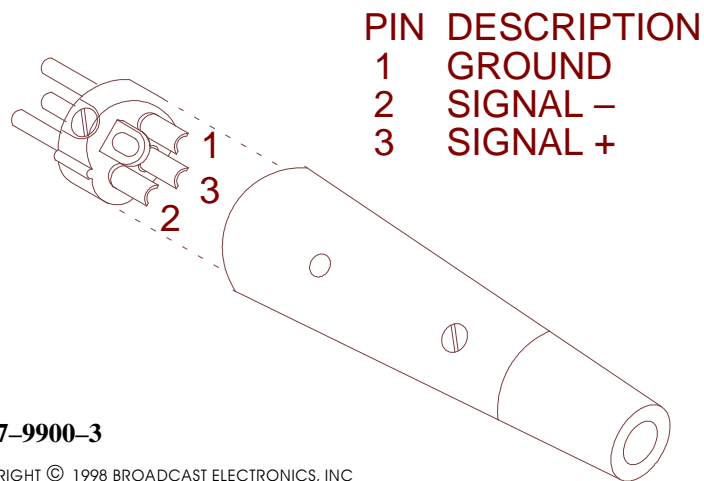
FIGURE 2. XLR PIN DESCRIPTIONS
