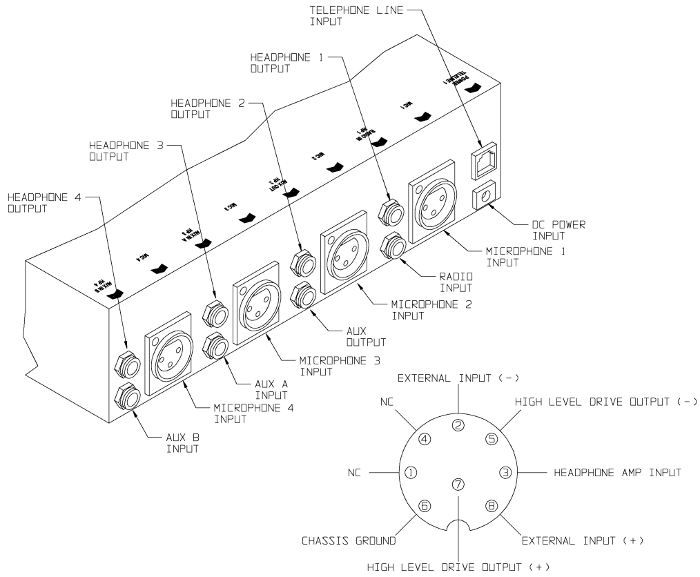
DIAGRAM #2 FRONT PANEL VIEW
